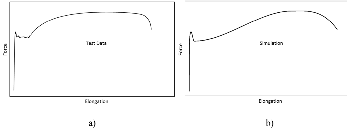
Figure 2: a) Actual Test Data (for a mild steel) and b) simulated Force – Elongation curve
